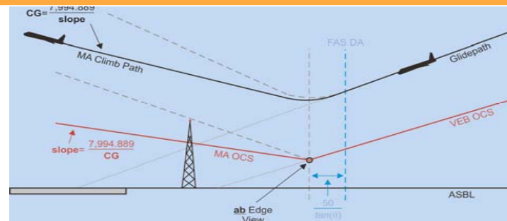
Vertical Profiles & Missed Approach
